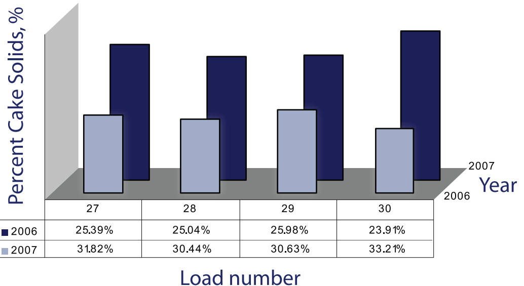
Graph showing nearly 20-40% increase in 2007 solids weight percent using THIOGUARD® over the same time in 2006 Lambertville, NJ - WWTP Biosolids
