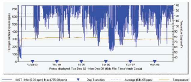
Pump Station with THIOGUARD® Feed @ ~68 GPD
