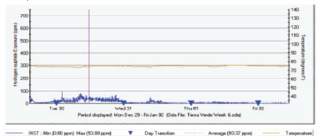
Pump Station with THIOGUARD® Feed @ ~32 - 36 GPD
